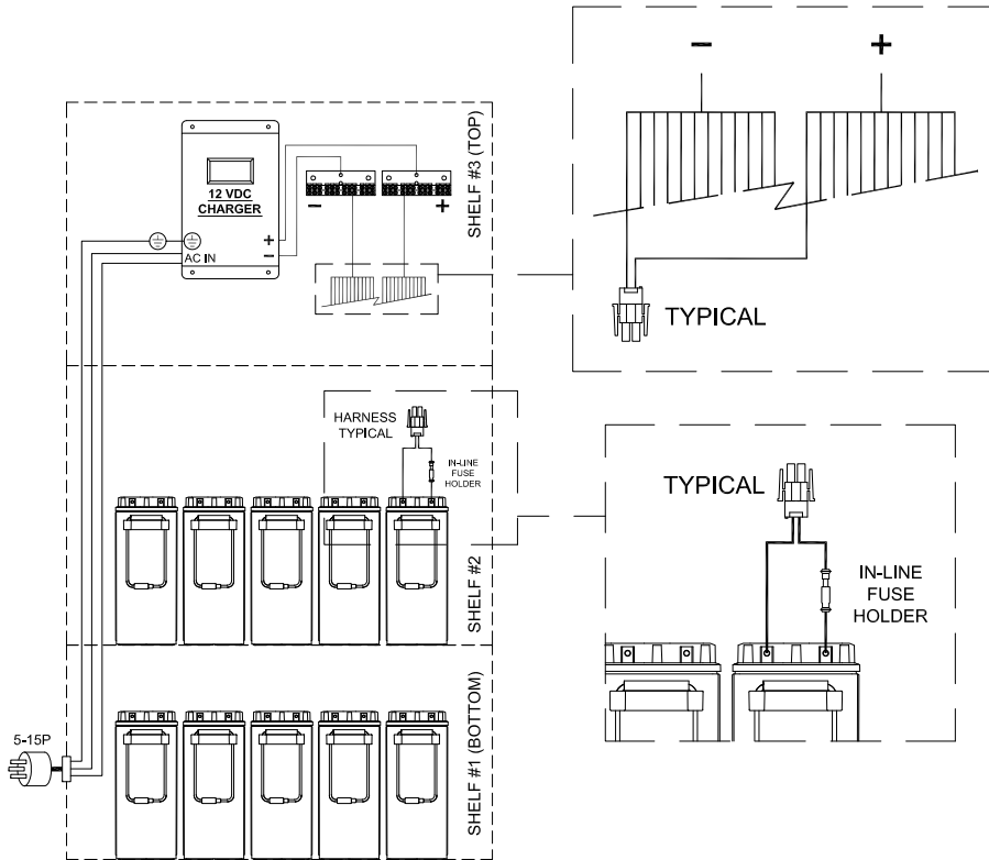
TYPICAL SPARES WIRING FOR (10) 150/170AH FRONT TERMINAL BATTERIES
