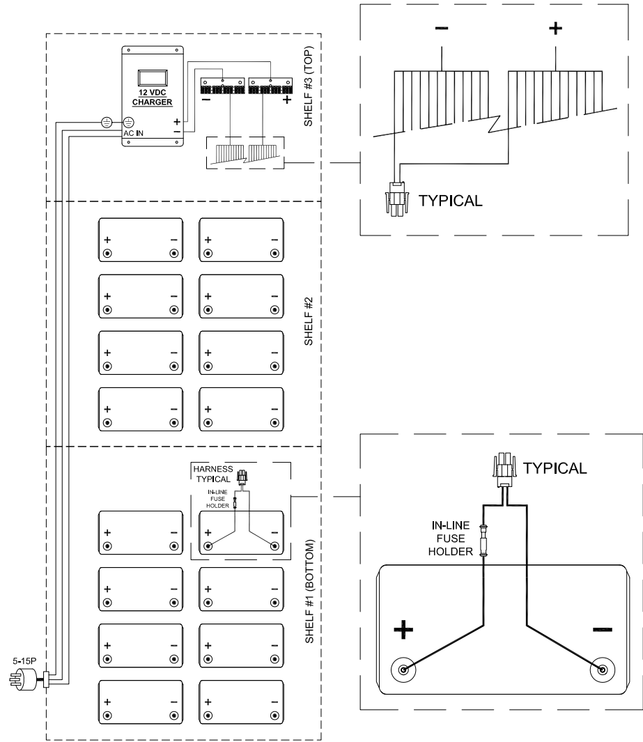
TYPICAL SPARES WIRING FOR (16) 540W TOP TERMINAL BATTERIES
