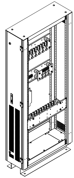
ISOMETRIC VIEW (COVERS REMOVED)
