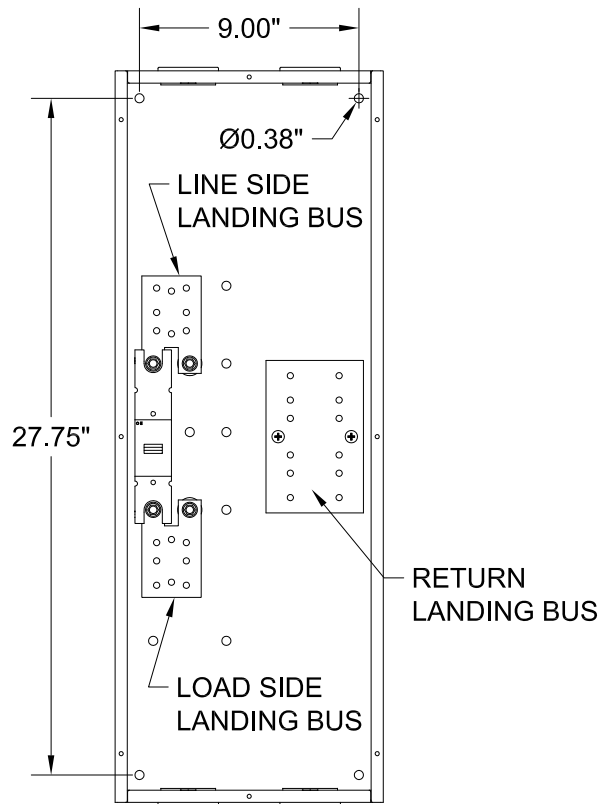
FRONT VIEW (COVER REMOVED)
