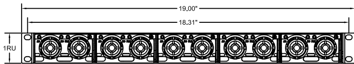
FRONT VIEW
